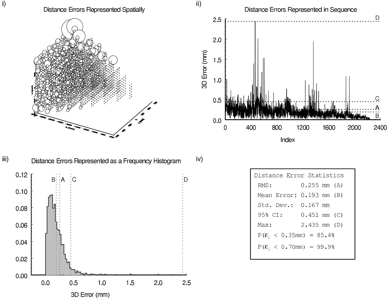
Figure 1. Typical distance error profiles for the Polaris position sensor at the time of characterization. The sequence of plots, from the full spatial representation in i) to the final statistical summary in iv), demonstrates how increasing simplicity and clarity come at the expense of continued loss of information. Plot i) represents the distance errors spatially at each reference position (x_r, y_r, z_r) , with the error magnitudes proportional to the corresponding circle diameters. In ii), the distance errors are plotted as a function of the sequence in which they were collected (from the back of the volume to the front). While the 3D spatial information has been lost, the general dependence of the error on the z -depth is still evident, as is the increased error at the edges. In iii), all of the spatial information has been lost, but the skewed non-Gaussian nature of the underlying error distribution is clearly evident (the distribution is related to the general Maxwell probability distribution that governs distance errors 4 ). The distance errors are then reduced to the statistical summary in iv), from which only one or two values (typically the overall volume RMS distance error) are presented to the user. These results are also tabulated in Table 2 and compared to other calibration results.
