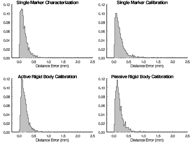
Figure 4. Frequency histograms for the distance errors shown in Table 2.
