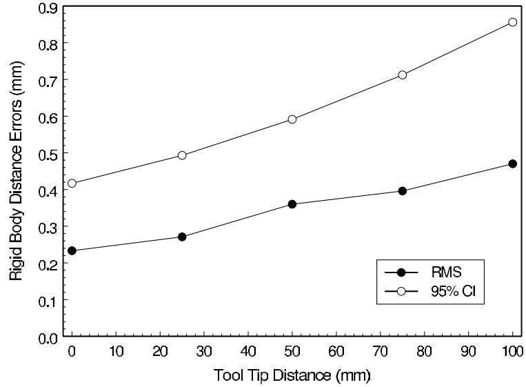
Figure 5. Inherent accuracy degradation of rigid body 3D positions as the tool tip distance is increased with respect to the rigid body markers. The RMS and 95% confidence interval accuracy results are presented for five different tool definitions. Each definition is identical, except that the tool tip position has been redefined to be at a different distance. The resulting accuracy values are plotted against this virtual tool tip length. The data were obtained from the active rigid body data shown in Table 2.
